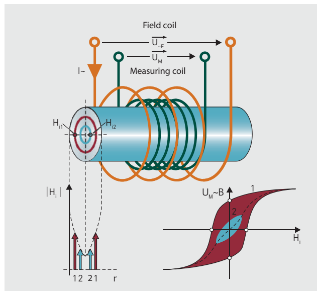
Scheme of magnetic inductive testing
